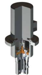
Gear Drive Section View
